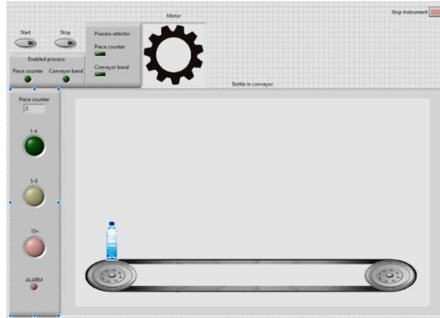
Figure 5 Elements of the front panel of the VI after adding animation frames.
