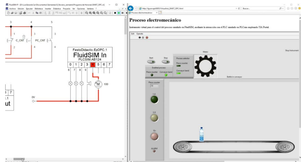
Figure 10 Execution of Process 2 in the plant and Web Services application.
